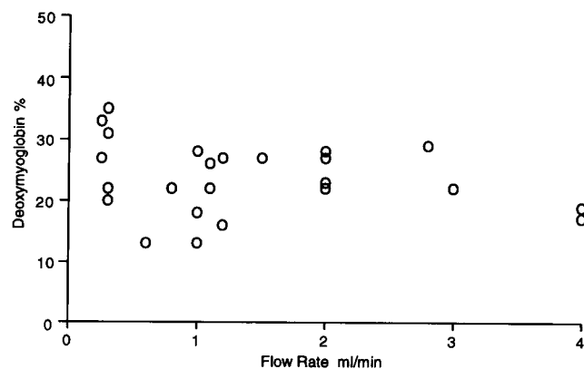
FIGURE 9 Scattergram showing the effect of increasing flow rate on deoxymyoglobin level in blood-perfused hearts. There is no correlation between flow rate, from 0.3 to 4.0 ml/min, and % myoglobin deoxygenation. The correlation coefficient R^2 = 0.063 ( n = 24 observations, six hearts).
