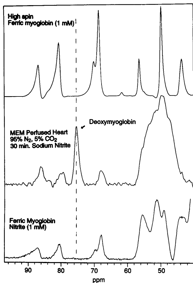
FIGURE 2 Comparison of ^1\text{H} NMR spectra of the MEM-perfused rat heart anaerobically perfused with sodium nitrite for 30 min with spectra of solutions of 1 mM high-spin ferric myoglobin and of 1 mM ferric myoglobin nitrite. Middle spectrum shows the spectrum of Fig. 1 e with expanded scale. 30% of the intracellular myoglobin is still in the deoxy form with its resonance at 76 ppm (-----). The rest of the intracellular myoglobin is converted to ferric myoglobin or its nitrite derivative, as indicated by the additional resonances near 50, 68, 81, and 87 ppm. Note that the deoxymyoglobin peak appears in a region where the spectra of both ferric myoglobin and ferric nitrite myoglobin are clear of spectral features. Horse met-myoglobin (1.0 mM, Sigma Chemical Co.) dissolved in 0.05 M Na-Hepes, pH 7.4 containing 0.5 mM EDTA was used to measure the top spectrum of high-spin ferric myoglobin. Sodium nitrite in large excess (200 mM) was added to this sample to convert ferric myoglobin to the nitrite derivative whose NMR spectrum is shown in the bottom trace.
