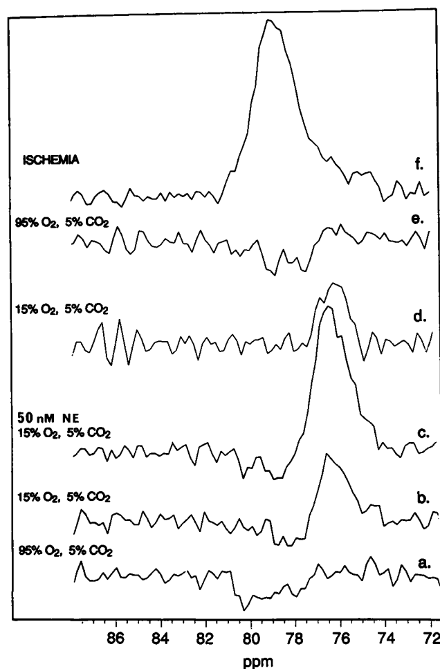
FIGURE 3 ^1\text{H} NMR spectra of an isovolumic MEM-perfused rat heart showing the reversible effect of perfusate deoxygenation and heart beat stimulation on the deoxygenation of intracellular myoglobin. Trace a shows the fully oxygenated control; myoglobin deoxygenation was vanishingly small, and heart rate was 400 bpm. Trace b shows that decreasing oxygenation of the perfusion medium to 15% oxygen from 95% decreased intracellular \text{P}_{\text{O}_2} and increased deoxymyoglobin to 31%. The heart rate was 185 bpm. The addition of 50 nM norepinephrine (NE) increased the heart rate from 185 to 400 bpm, which would be expected to increase the oxygen consumption of the heart. Trace c shows that the deoxymyoglobin resonance increased to 77% with norepinephrine indicating that the intracellular \text{P}_{\text{O}_2} decreased, (to 1 torr from 6 torr). One h later, the heart rate dropped again to 185 bpm, and deoxymyoglobin decreased to 20% (trace d , \text{P}_{\text{O}_2} = 10 torr) comparable to that observed before norepinephrine treatment at this level of medium oxygenation 2 h earlier (trace b ). Increasing medium oxygenation to 95% oxygen again lowered the deoxymyoglobin resonance to negligible levels, even though heart rate had dropped to 130 bpm (trace e ). The final no-flow ischemia spectrum is shown in trace f .
